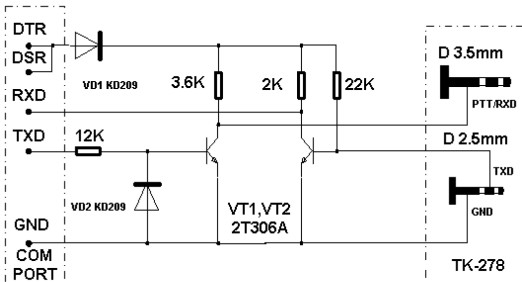
programming cable for KG-UVD1/P
