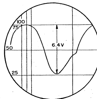
(E) WAVEFORM AT GRID PIN 7, V701
