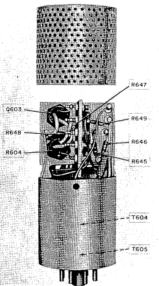
Figure 38. Audio module, right side view, cover removed.
