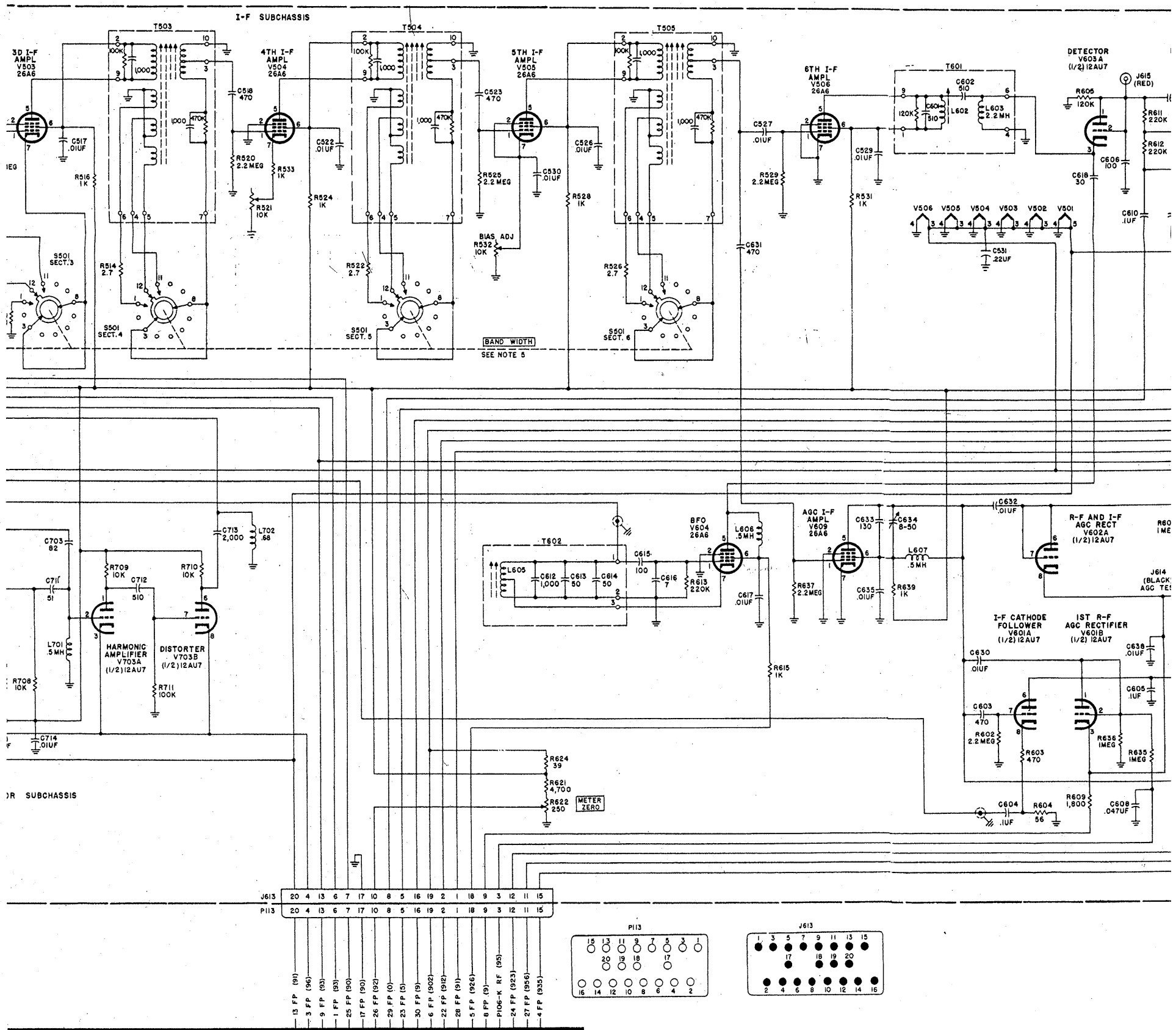
Figure 82(2). Radio receiver, wiring diagram (part 2 of 2).
