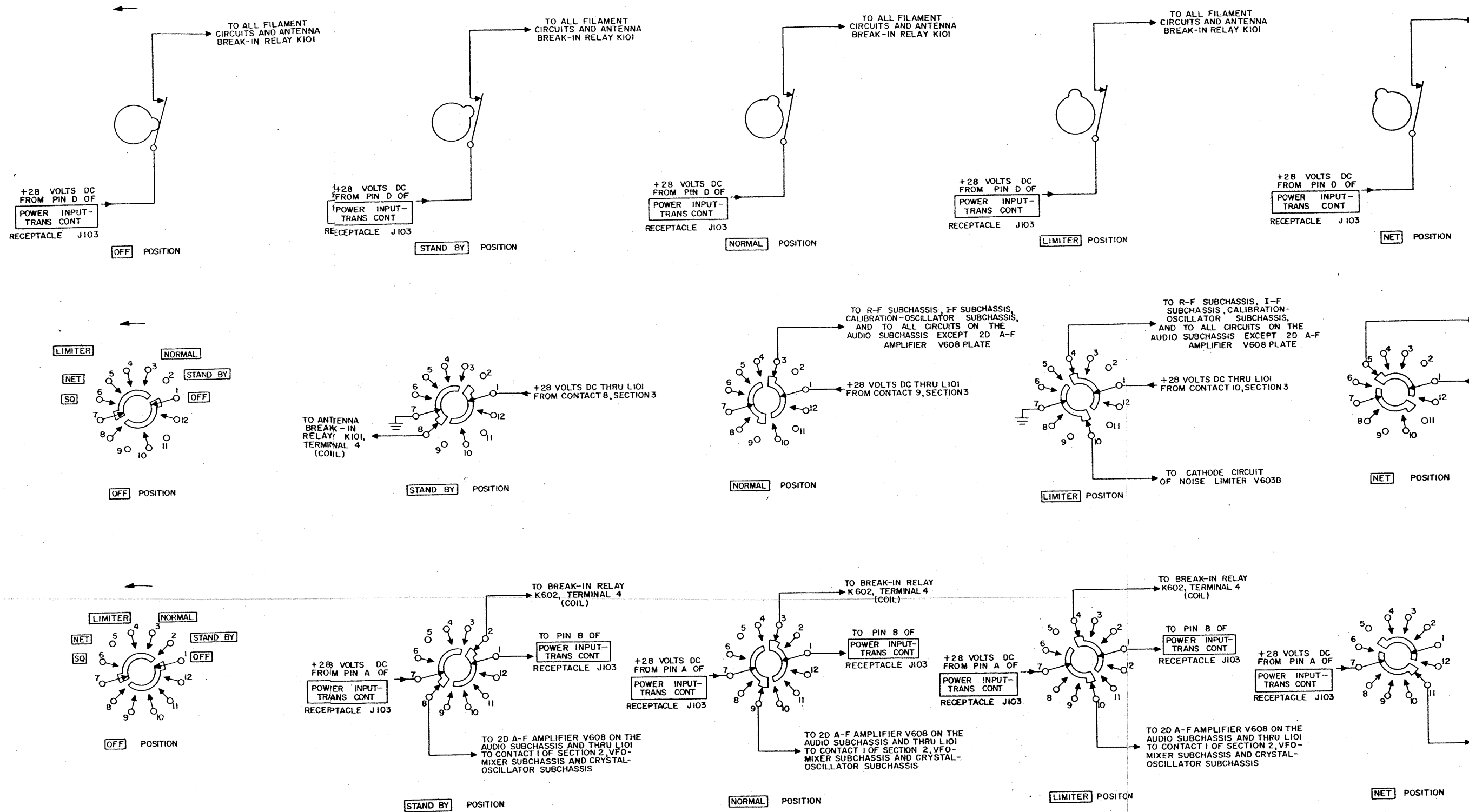
Figure 26. Function switch S104, schematic diagram.
