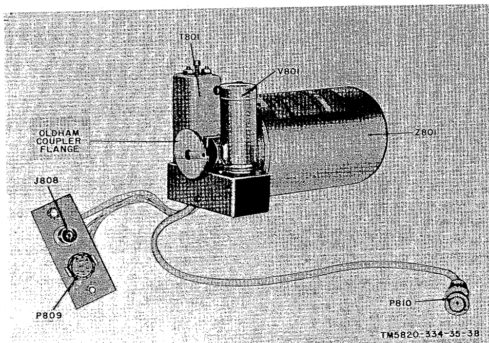
Figure 41. Vfo subchassis.
