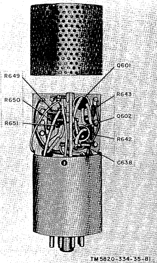
Figure 37. Audio module, left side view, cover removed.
