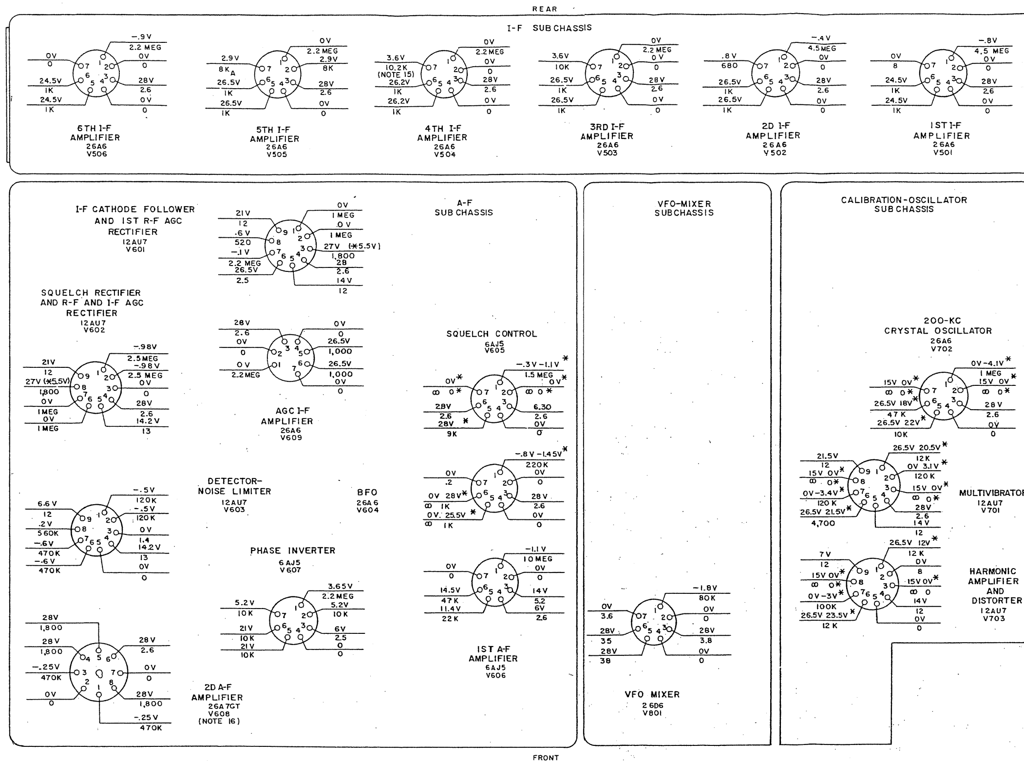
Figure 79. Lower deck, voltage and resistance diagram.
