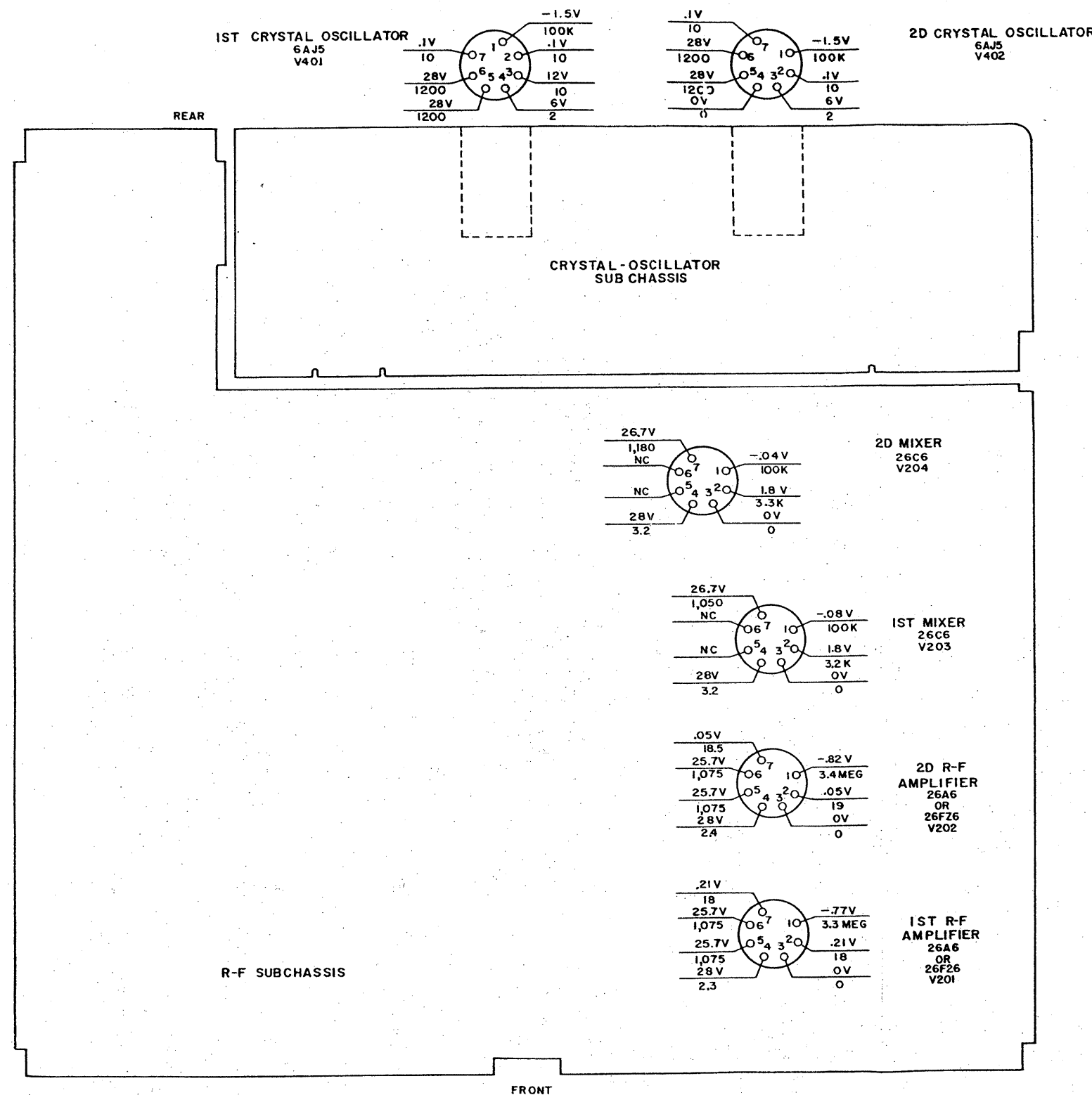
Figure 78. Upper deck, voltage and resistance diagram.
