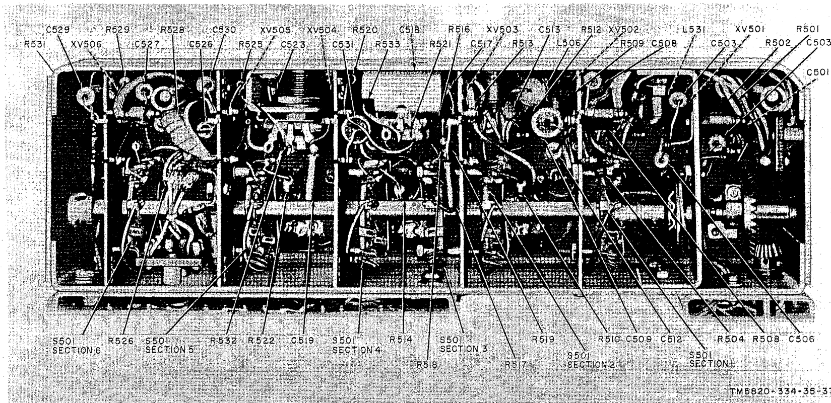
Figure 40. If. subchassis, bottom view.
