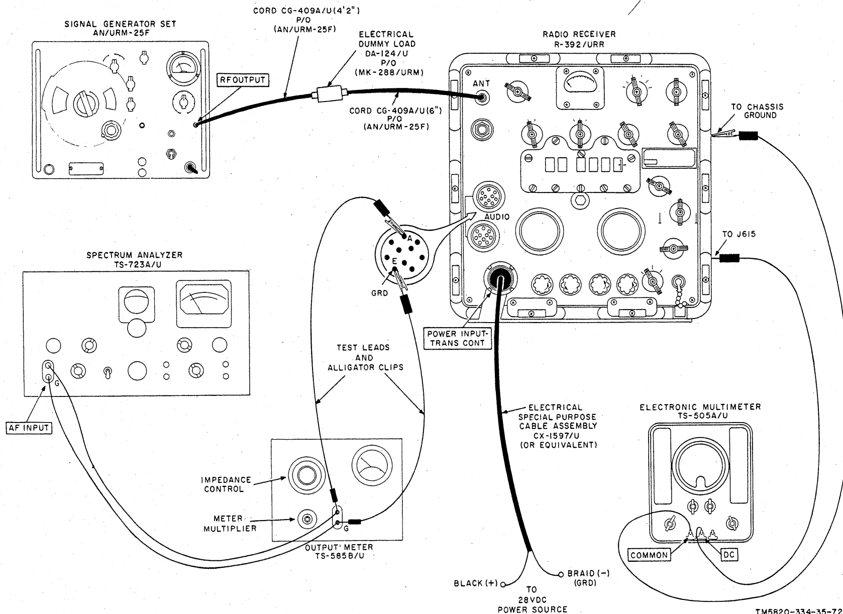
Figure 72. Distortion test.
