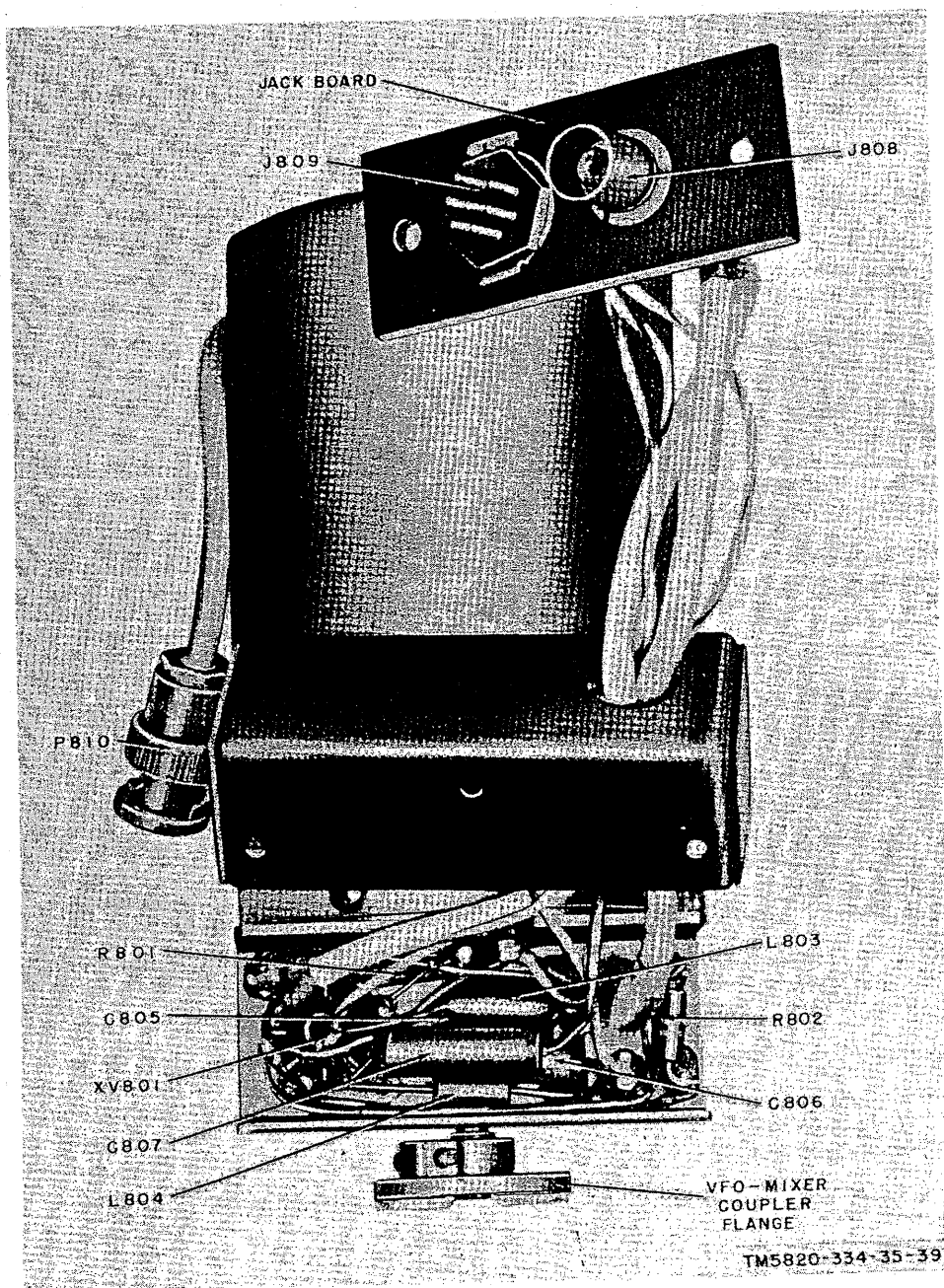
Figure 42. Vfo subchassis, bottom cover removed.
