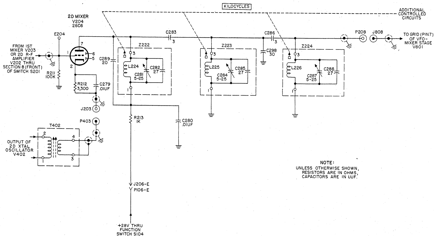
Figure 6. Second mixer V204, simplified schematic diagram.
