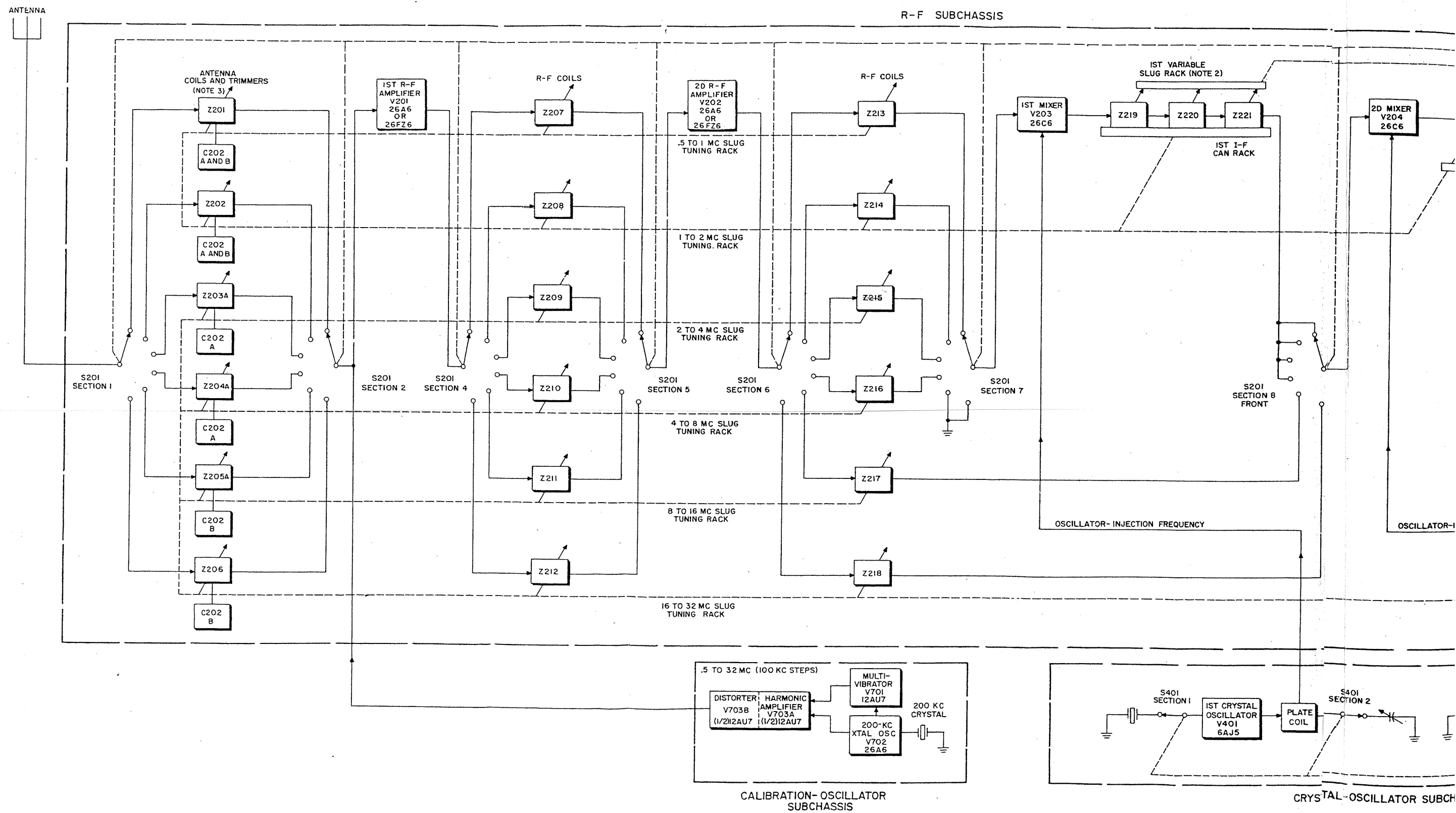
Figure 30. Tuning system, functional block diagram.
