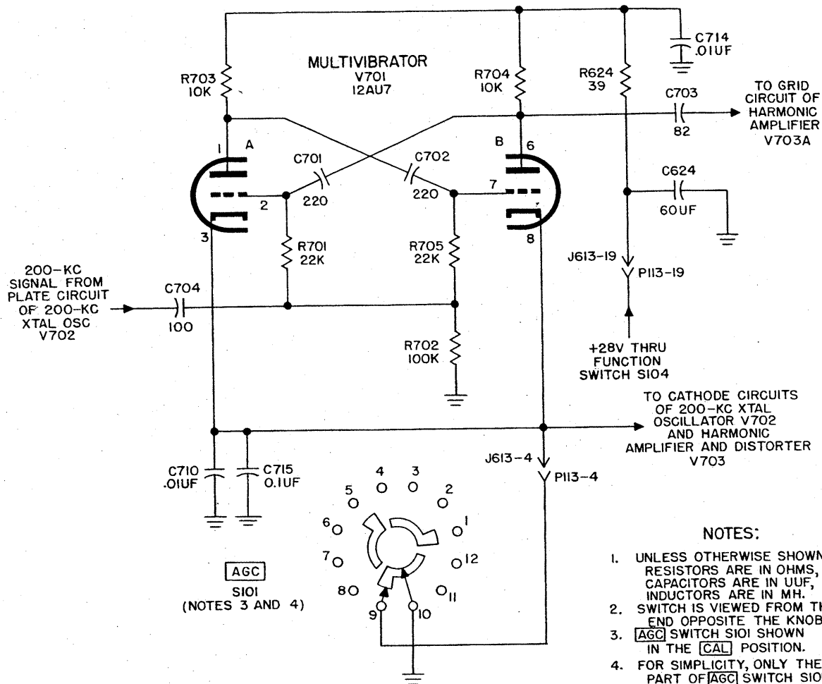
Figure 23. Multivibrator V701, simplified schematic diagram.
