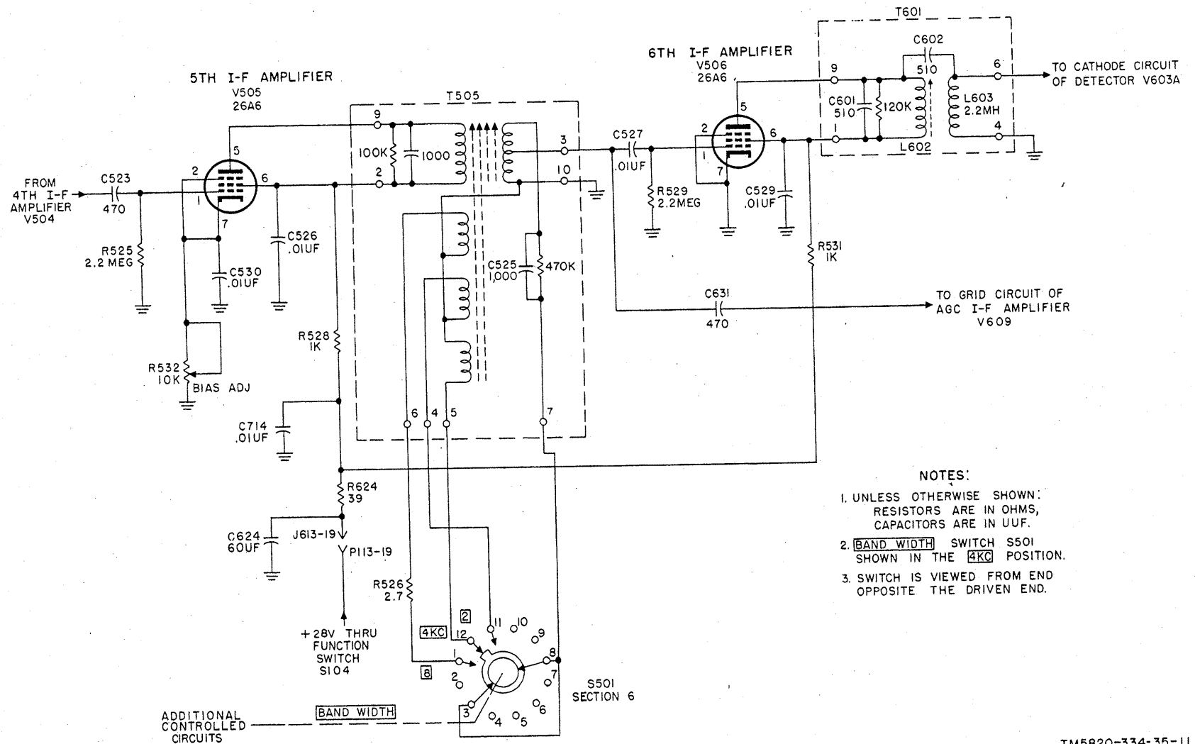
Figure 11. Fifth and sixth if. amplifiers V505 and V506, simplified schematic diagram.
