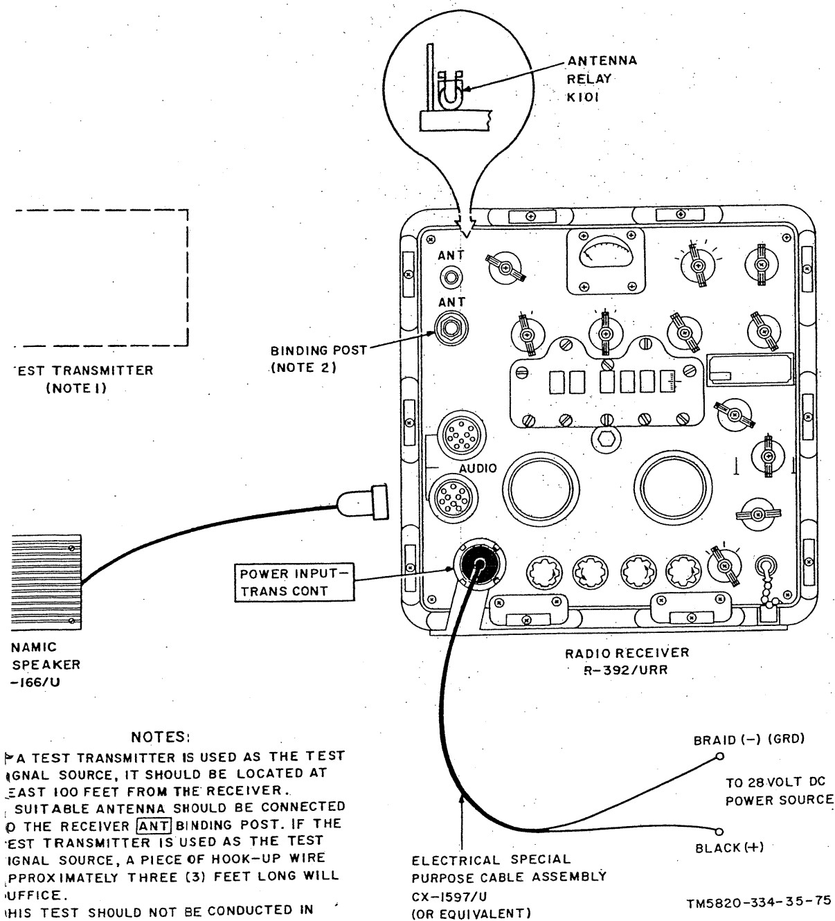
Figure 76. Operational test.
