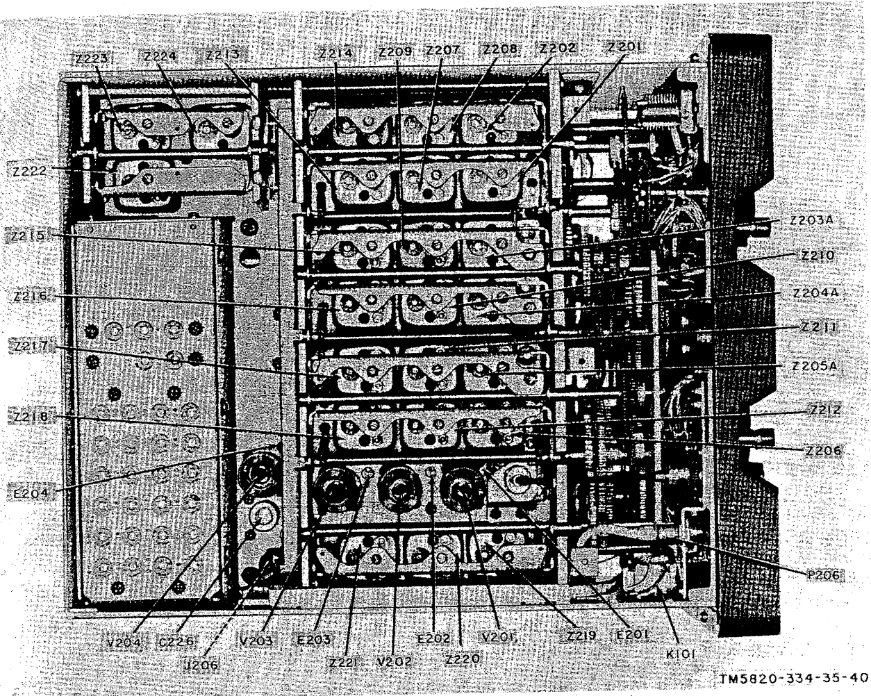
Figure 43. Upper deck assembly, top view.
