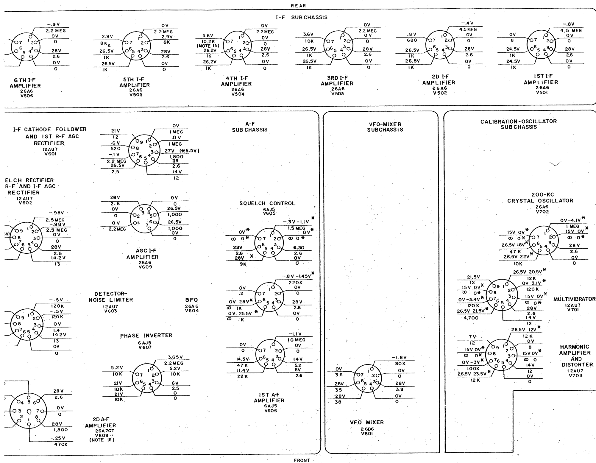
Figure 79. Lower deck, voltage and resistance diagram.
