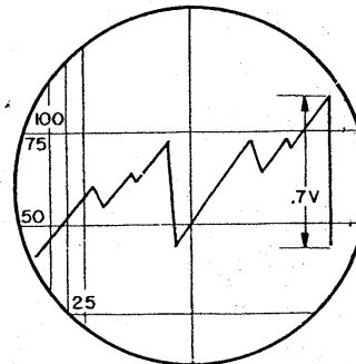
(L) WAVEFORM AT PLATE PIN 6, V703
