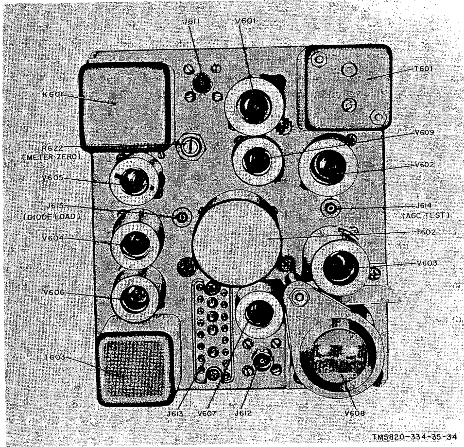
Figure 35. Audio subchassis, top view.
