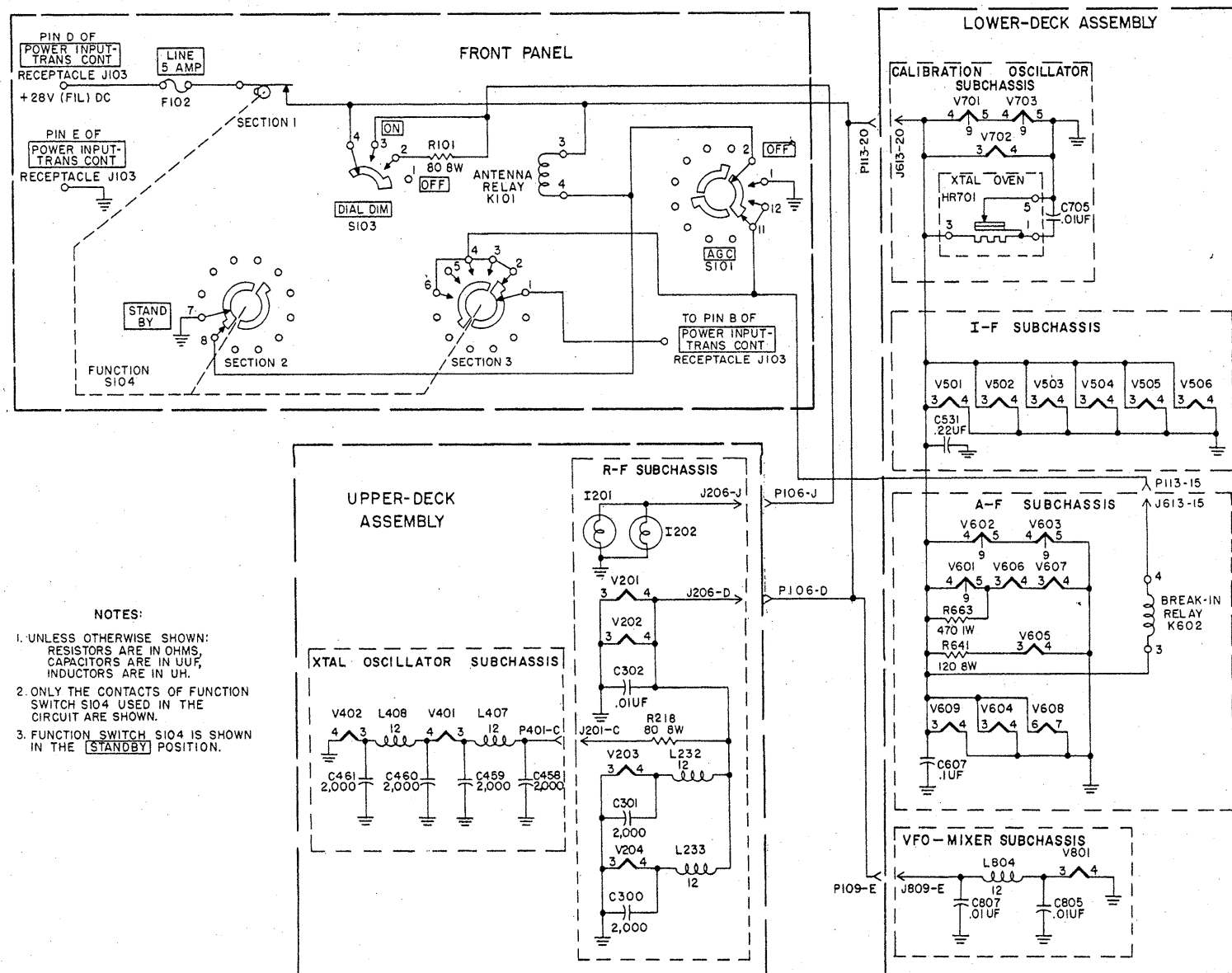
Figure 25. Filament and oven-heater circuits, simplified schematic diagram.
