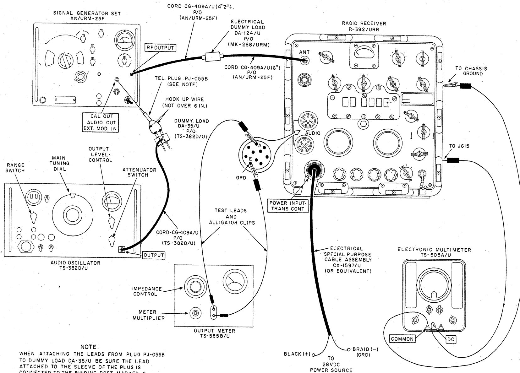
Figure 71. Overall audio response test.
