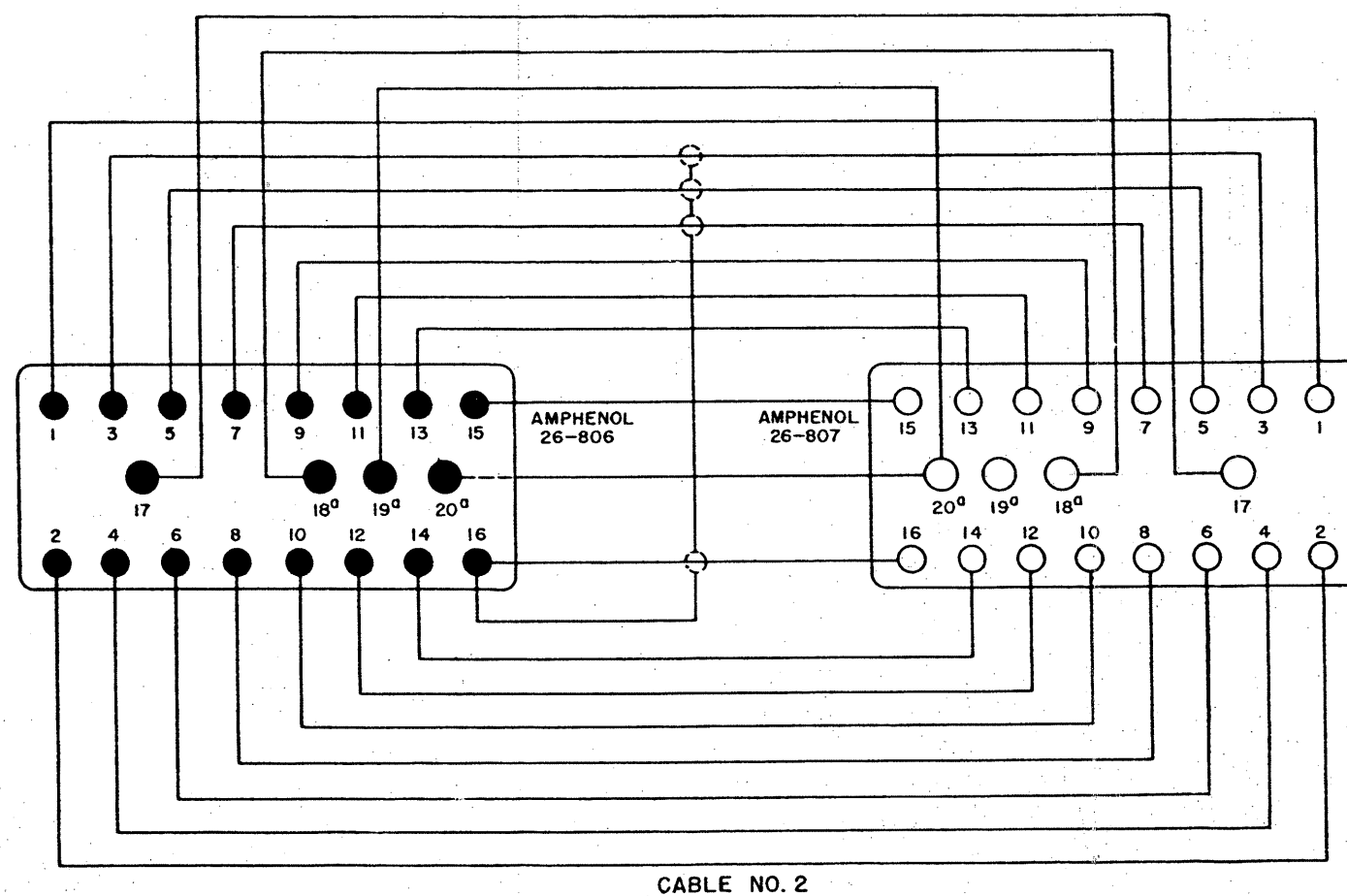
Figure 34. Cable No. 2, 3, and 4, assembly instructions.
