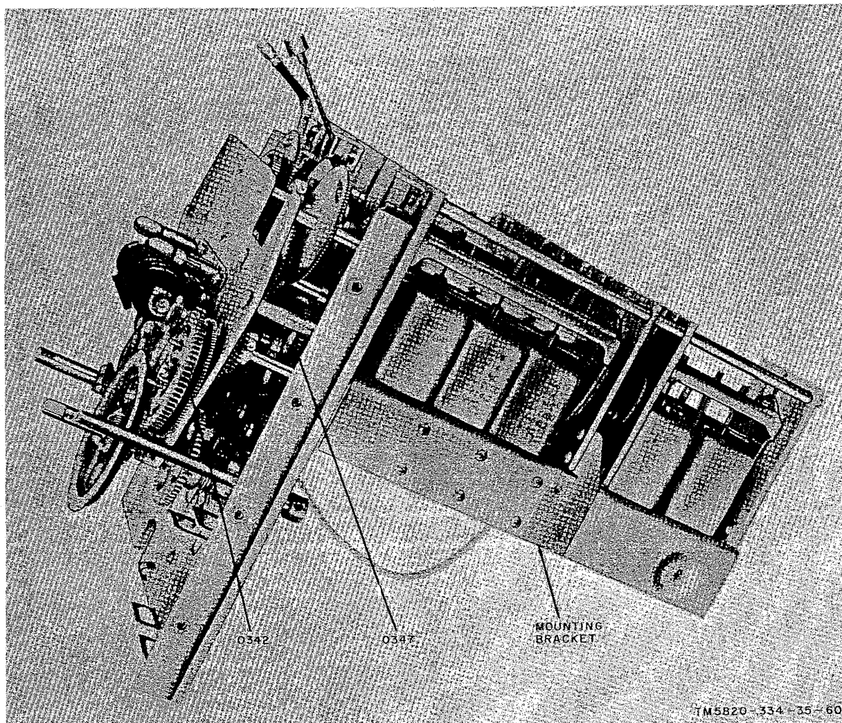
Figure 62. Gear train assembly and rf subchassis, right view.
