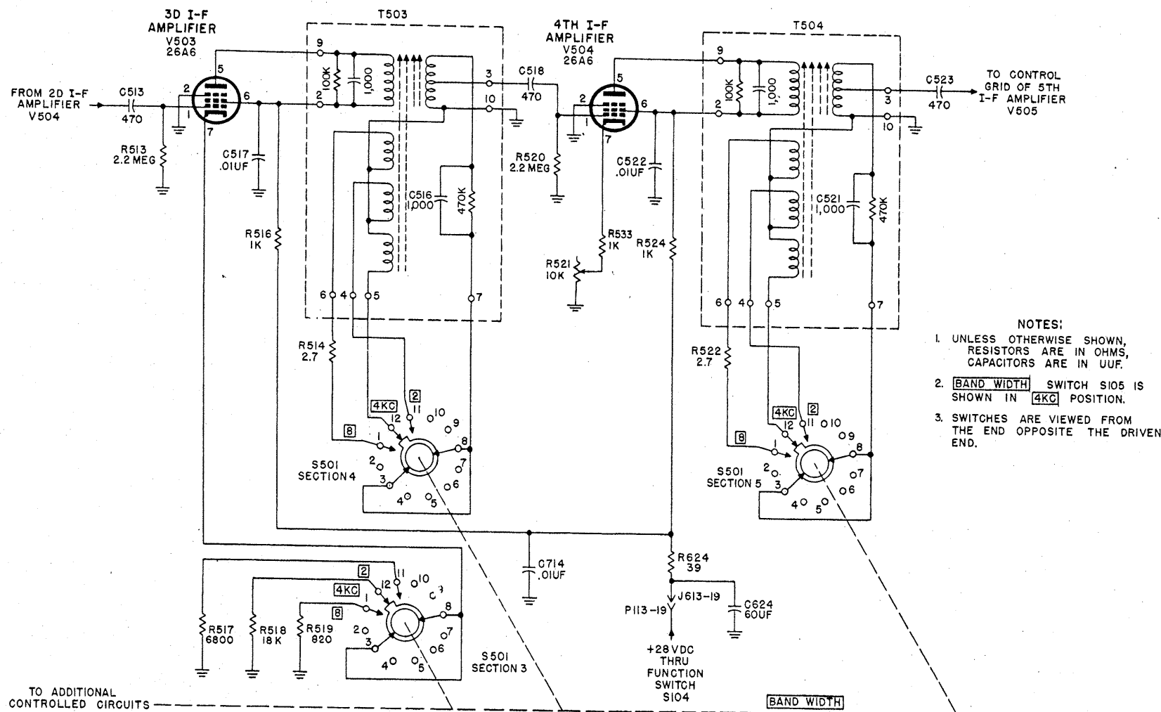
Figure 10. Third and fourth if. amplifiers V503 and V504, simplified schematic diagram.
