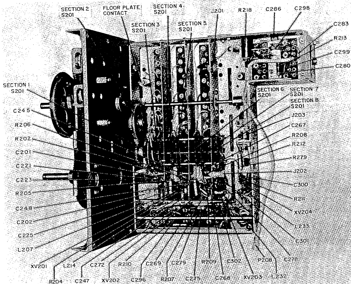
Figure 44. Upper deck assembly, bottom view.
