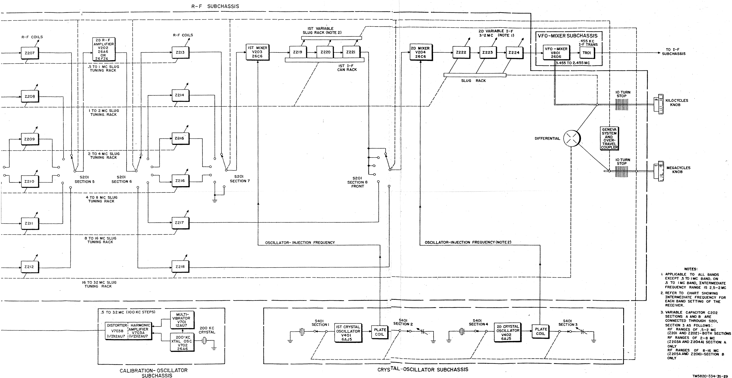
Figure 30. Tuning system, functional block diagram.
