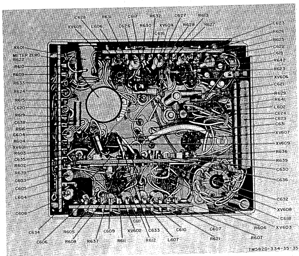
Figure 36. Audio subchassis, bottom view.
