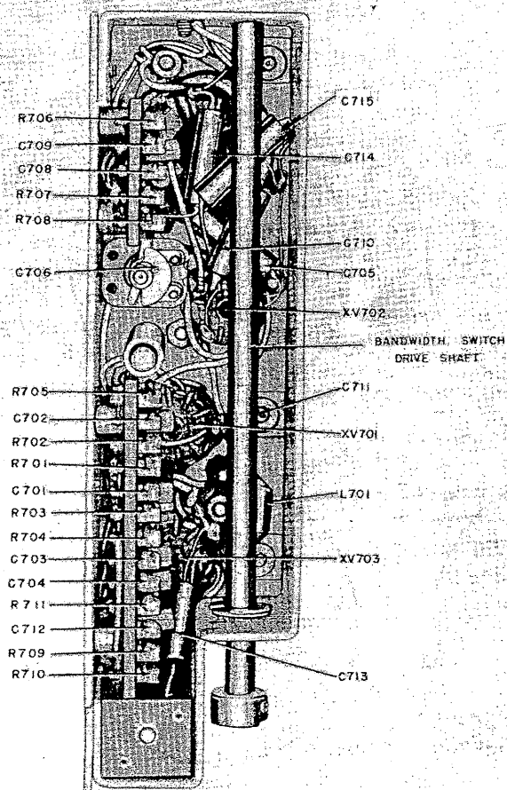
Figure 51. Calibration oscillator subchassis, bottom view.
