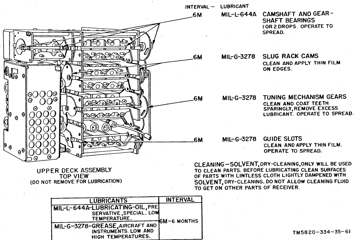
Figure 63. Radio Receiver R-392/URR, lubrication.
