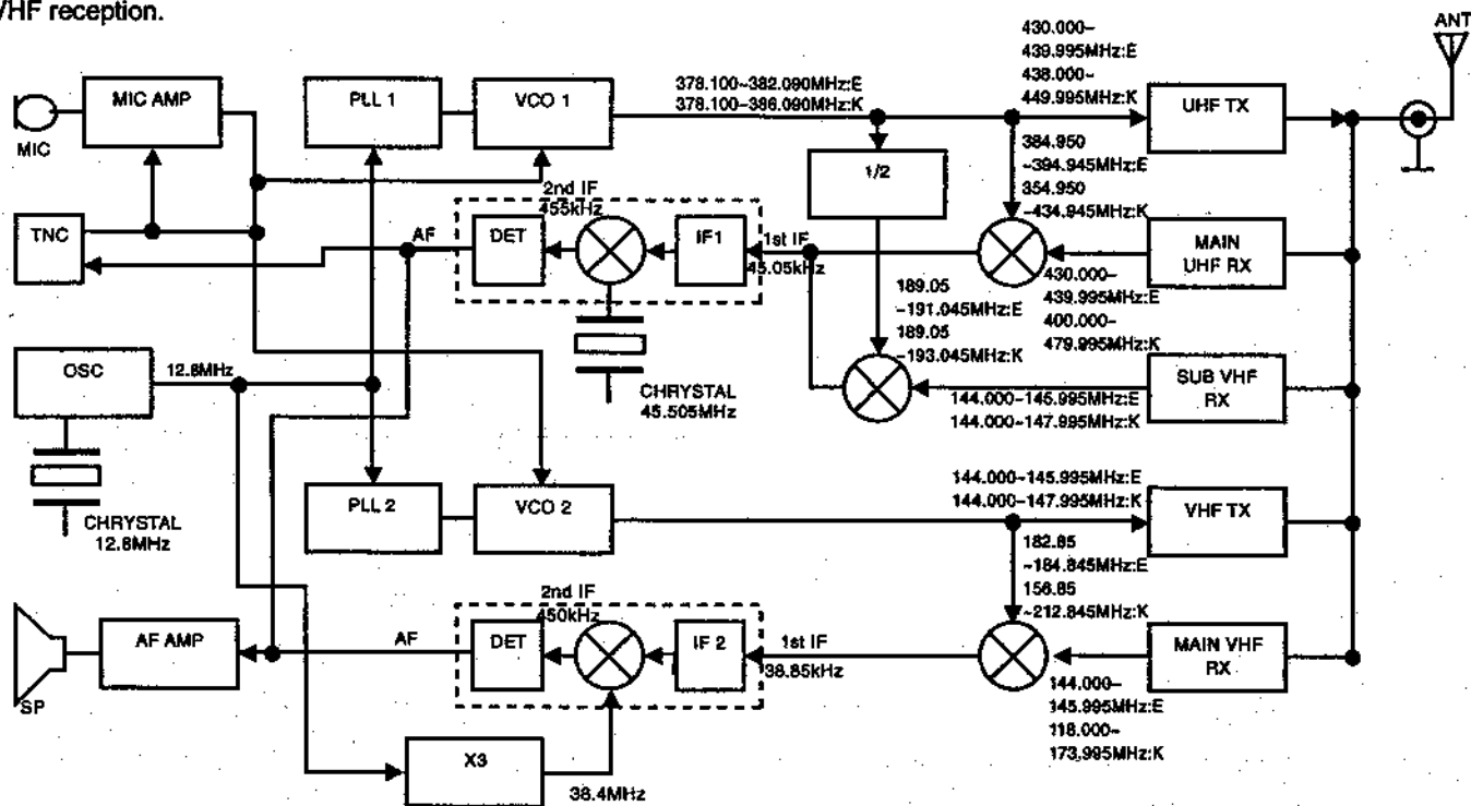
Fig.1 Frequency Configuration
