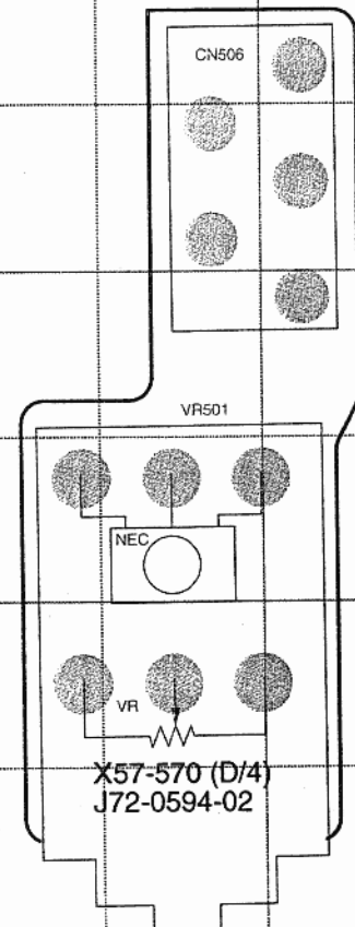
VOL, ENC UNIT (X57-570X-XX) (D/4) Foil Side View
