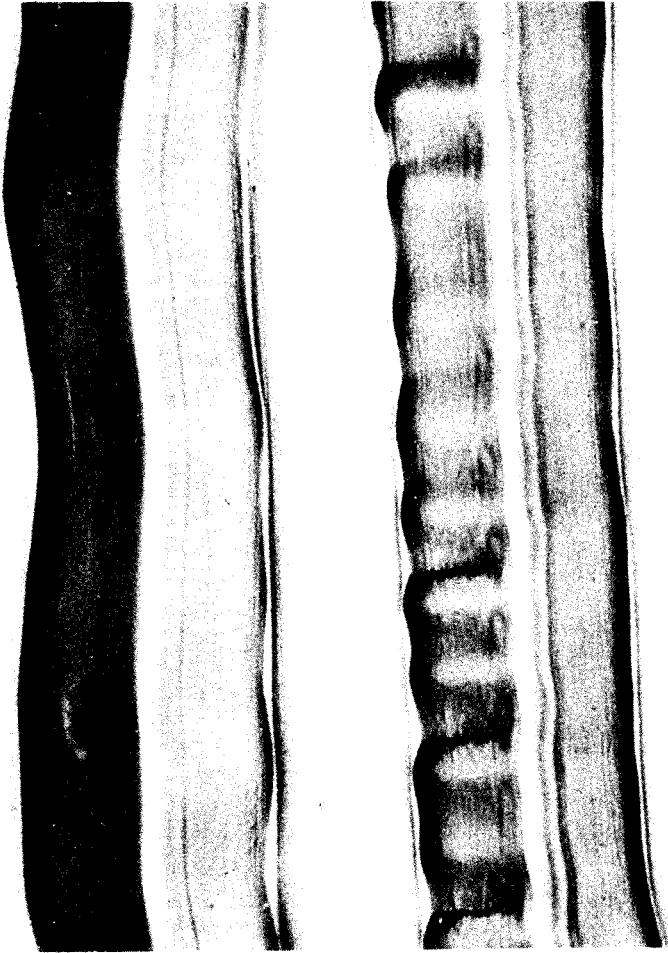
FIG. R/16. Groove after 165 playings showing little wear. Mag. 300x.
