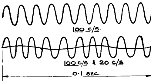
FIG. F/3. Effect of 20 cycle flutter on 100 c/s pure tone.
