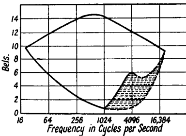
FIG. D/3. Auditory chart of a person deaf to high frequencies. Also from Wave Motion and Sound .
