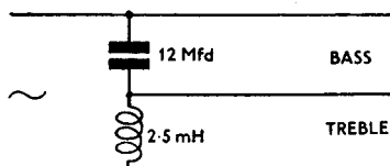
N.W.4. Quarter Section, Series
