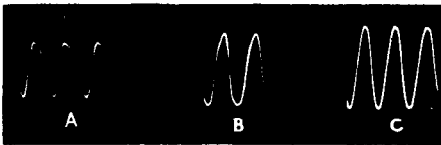
FIG. N/1. Non-linearity at A and B at 40 c/s with 1 watt input to 10" unit. A—Corrugated paper surround. B—Cloth surround. C—Foam plastic surround.
