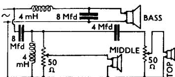
N.W.9. Half Section, 3-speaker circuit. Crossover at 800 and 5,000 c/s.
