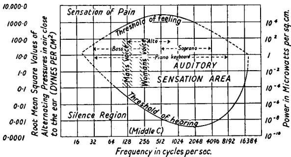
From Wave Motion and Sound by Stephens and Bate. Arnold. FIG. D/2. Working limits of the ear for pure tones.
