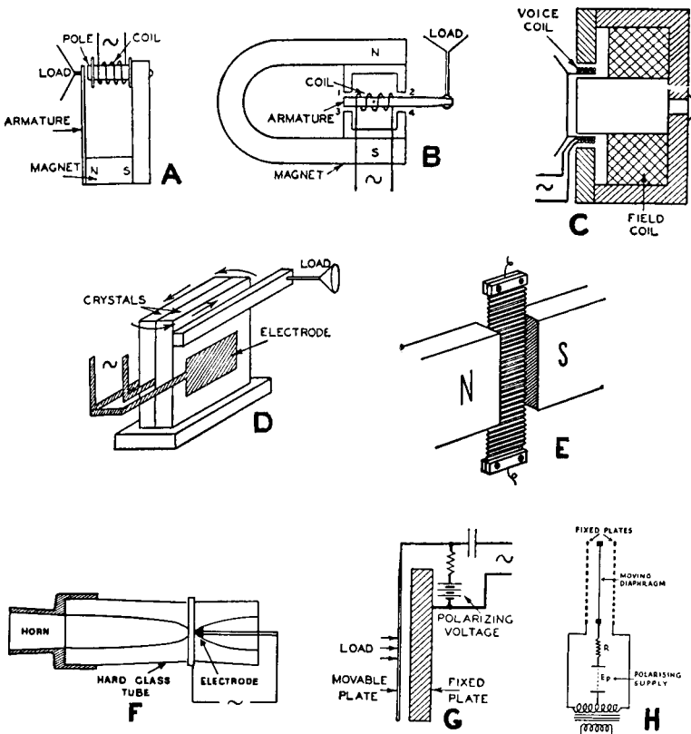
FIG. L/5. Driving Systems.
