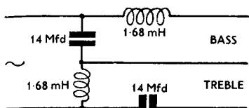
N.W.5. Half Section, Series
