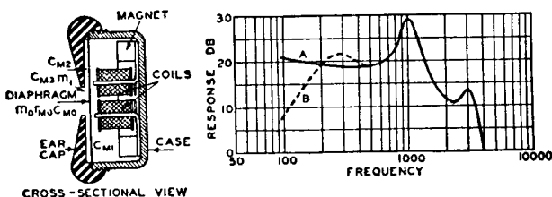
FIG. E/1. Diagram and response curve of magnetic earphone, taken from Olson's Elements of Acoustical Engineering .
