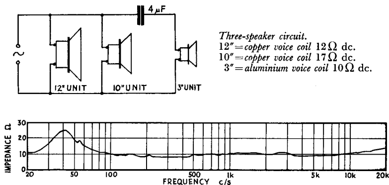
FIG. I/2. Unusually level impedance curve achieved by parallel working.
