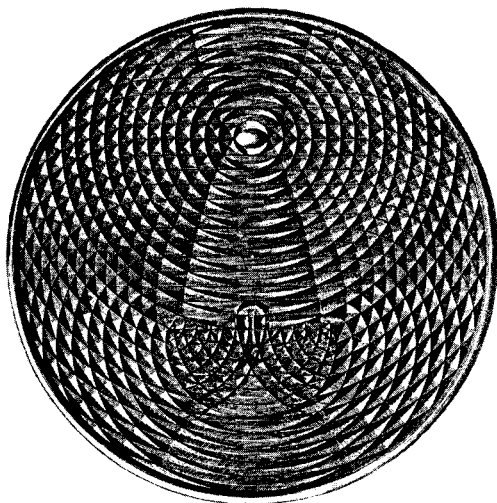
FIG. S/3. Ripples on the surface of water which are similar to sound waves.
