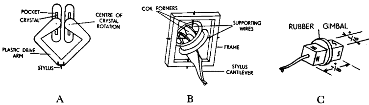
FIG. C/1. Cantilevers in stereo pickups.
