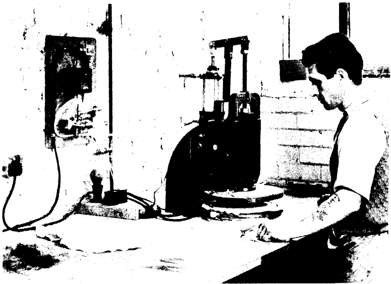
FIG. R/19B. Pneumatically operated and timed moulding press.
