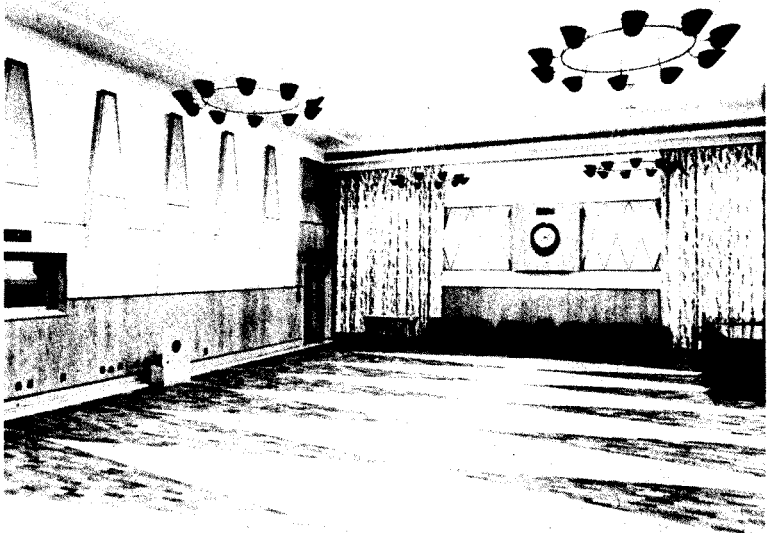
FIG. C/15. Maida Vale Studio 3, showing acoustic curtains in background and absorbent panels of special shape on side walls and ceiling. The wooden panelling near the floor provides low frequency absorption. Note baffle mounted talk-back speaker on the left.
