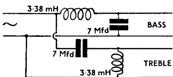
N.W.6. Half Section, Parallel
