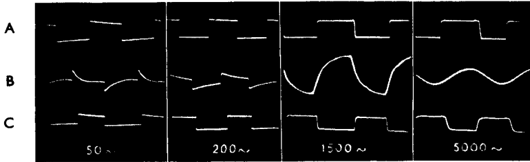
FIG. S/4A. Square waves at 50, 200, 1,500 and 5,000 c/s.
