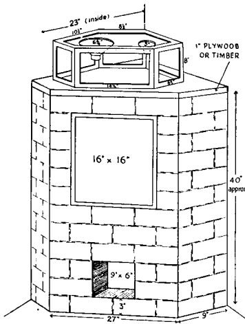
FIG. B/3. Brick corner enclosure, 9 cu.ft., used with no interior lining or absorbers.
