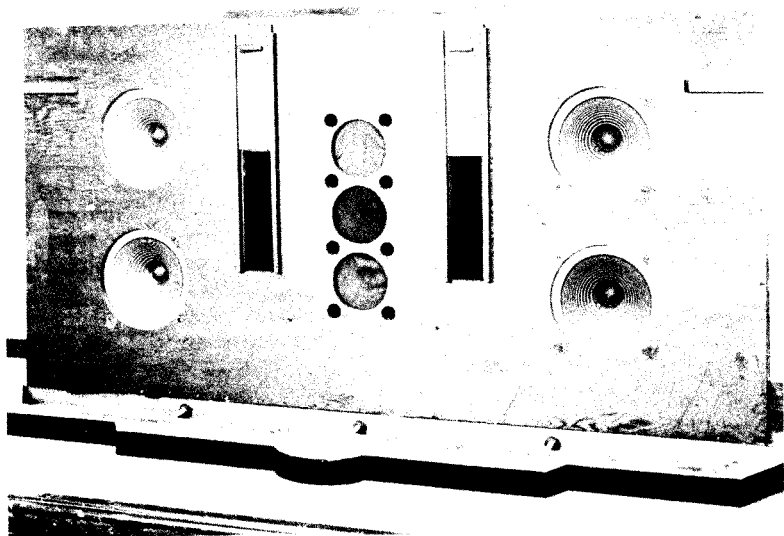
FIG. O/1. Loudspeaker system for electronic organ. Courtesy J. Wood & Sons Ltd., Huddersfield.
