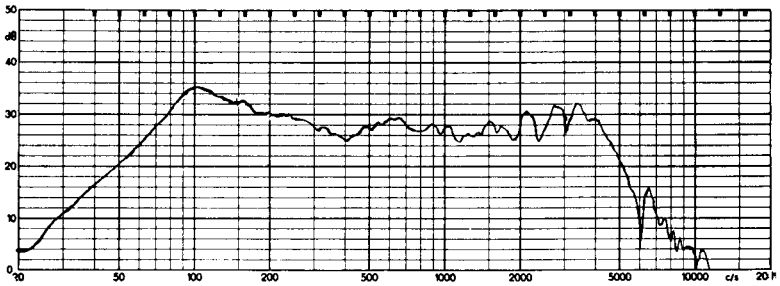
FIG. L/7. Axial response of 1930 model. Bass resonance 90 c/s.
