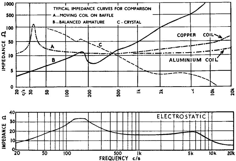
FIG. I/1. Typical impedance curves.
